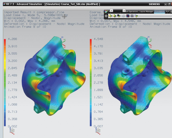
Analysis/analysis correlation, compressor part, different meshes, side-by-side animation.
