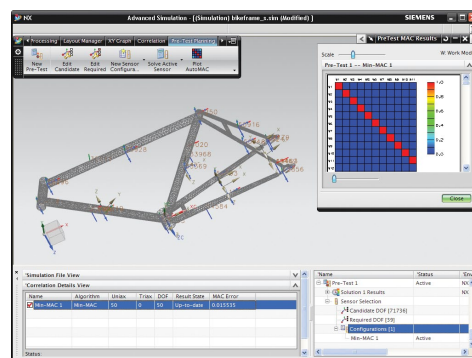
Pretest planning, selected sensors and autoMAC display.
