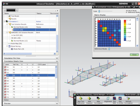
Test/analysis model overlay with sensors and MAC.
